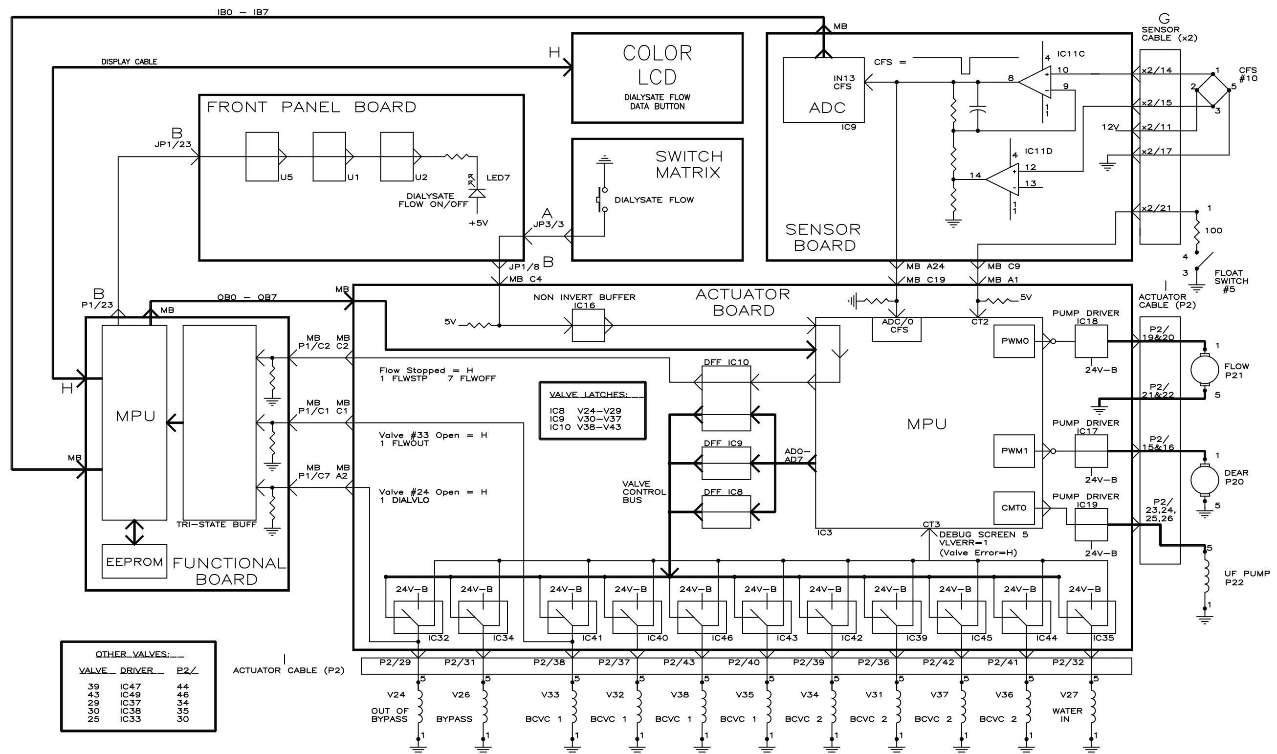
DIAGRAM C FLOW
